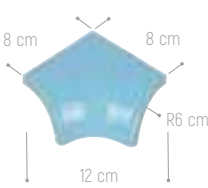
REF. 342 ÁNGULO INTERIOR ARISTA 12 x 8 x 8 cm - 4.7 "x3.1" x 3.1"
